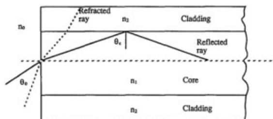
Figure 2. Basic Geometry of Optical Fiber Sensor
